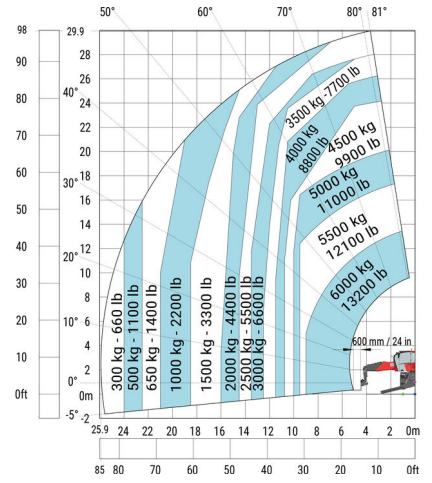
Machine on lowered stabilisers with 6000 kg jib (Metric)
